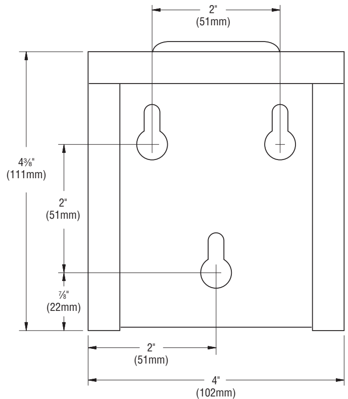
Bracket Mounting
