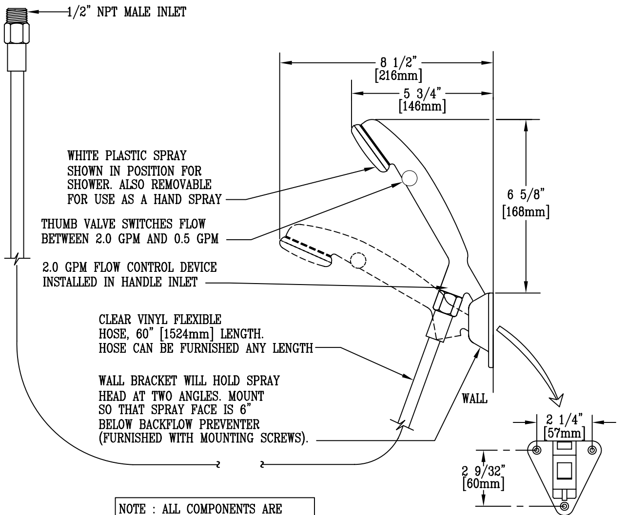
WALL BRACKET MOUNTING DETAIL
