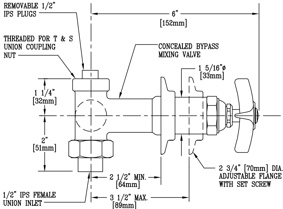
SIDE VIEW
