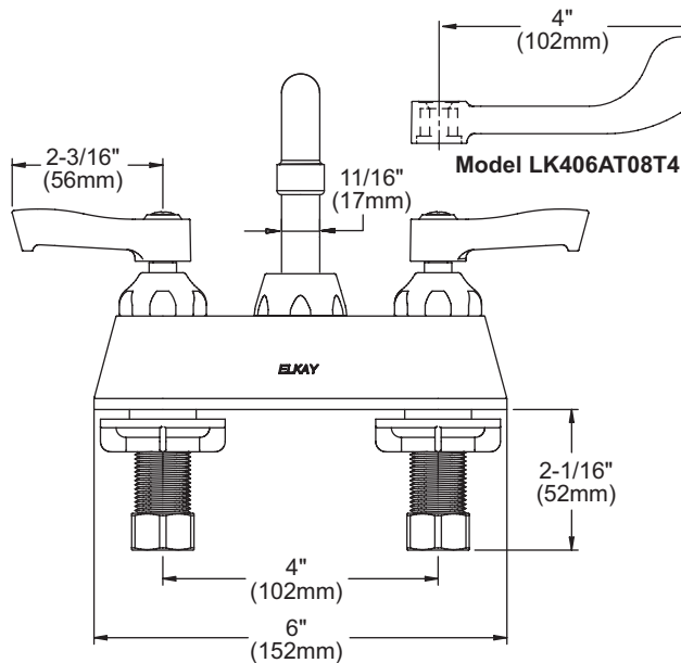
Model LK406AT08L2 FRONT VIEW
