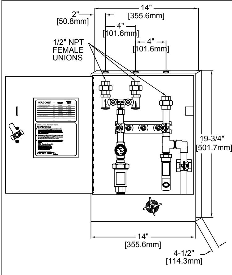
EXPOSED MOUNTING
