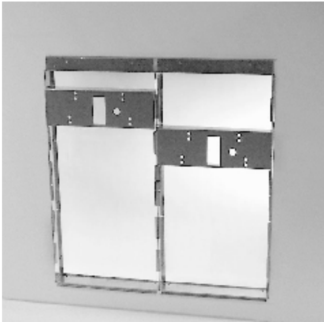
Figure 6 – HTSER-Q Rough-In
